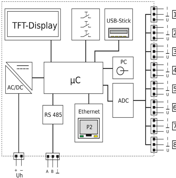
Fig. 2: Block diagram
