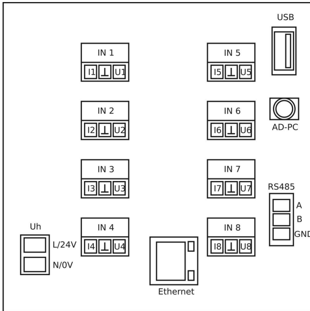
Fig. 9: Pin assignment rear view of product
